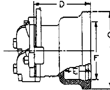
F-3004 Hub End Frame
